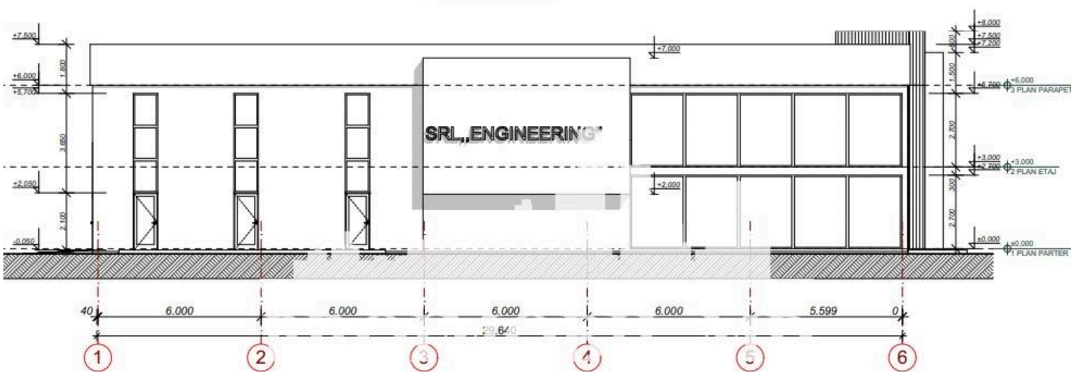
FATADA in axele 1-6 Sc. 1:100 (dimensiuni constructive)
